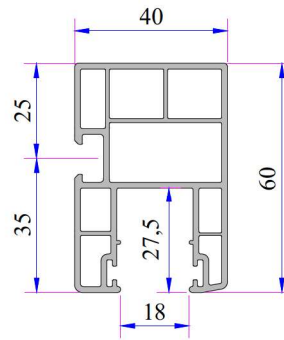
55'lik Lamel Yan Ray Kod: P.A.097.5613.600.0.00.19
